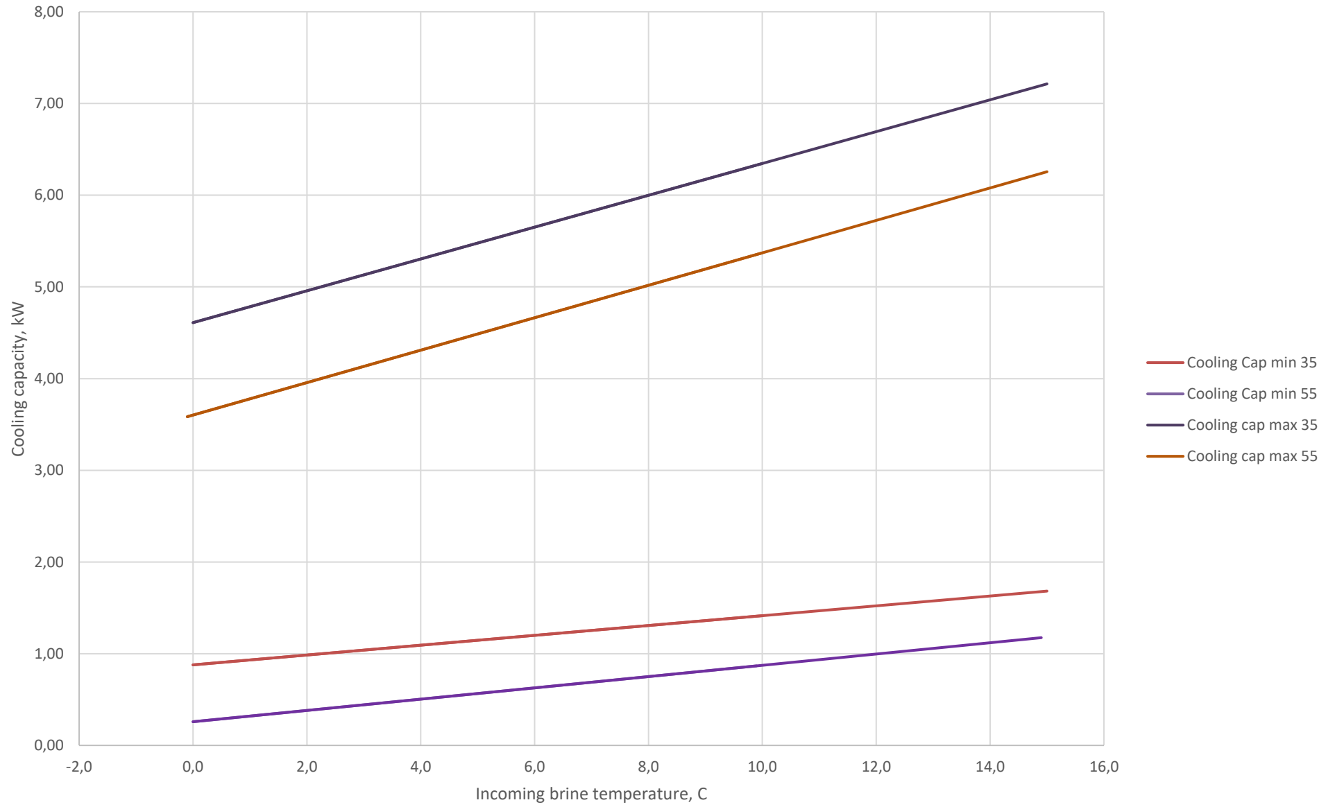
Cooling capacity S1X55-6
