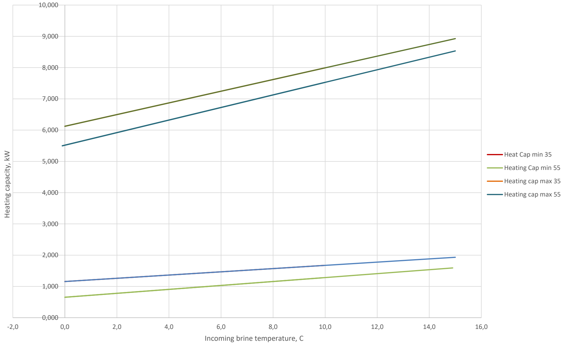
Heating capacity S1X55-6
