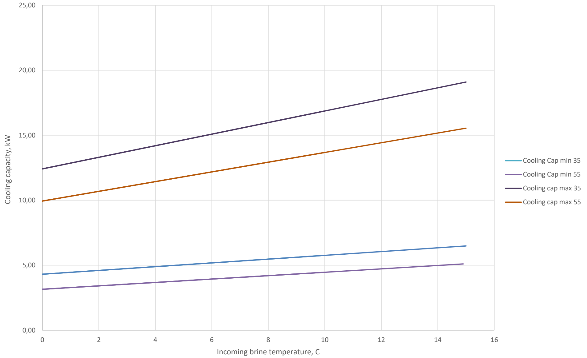
Cooling capacity S1X55-16
