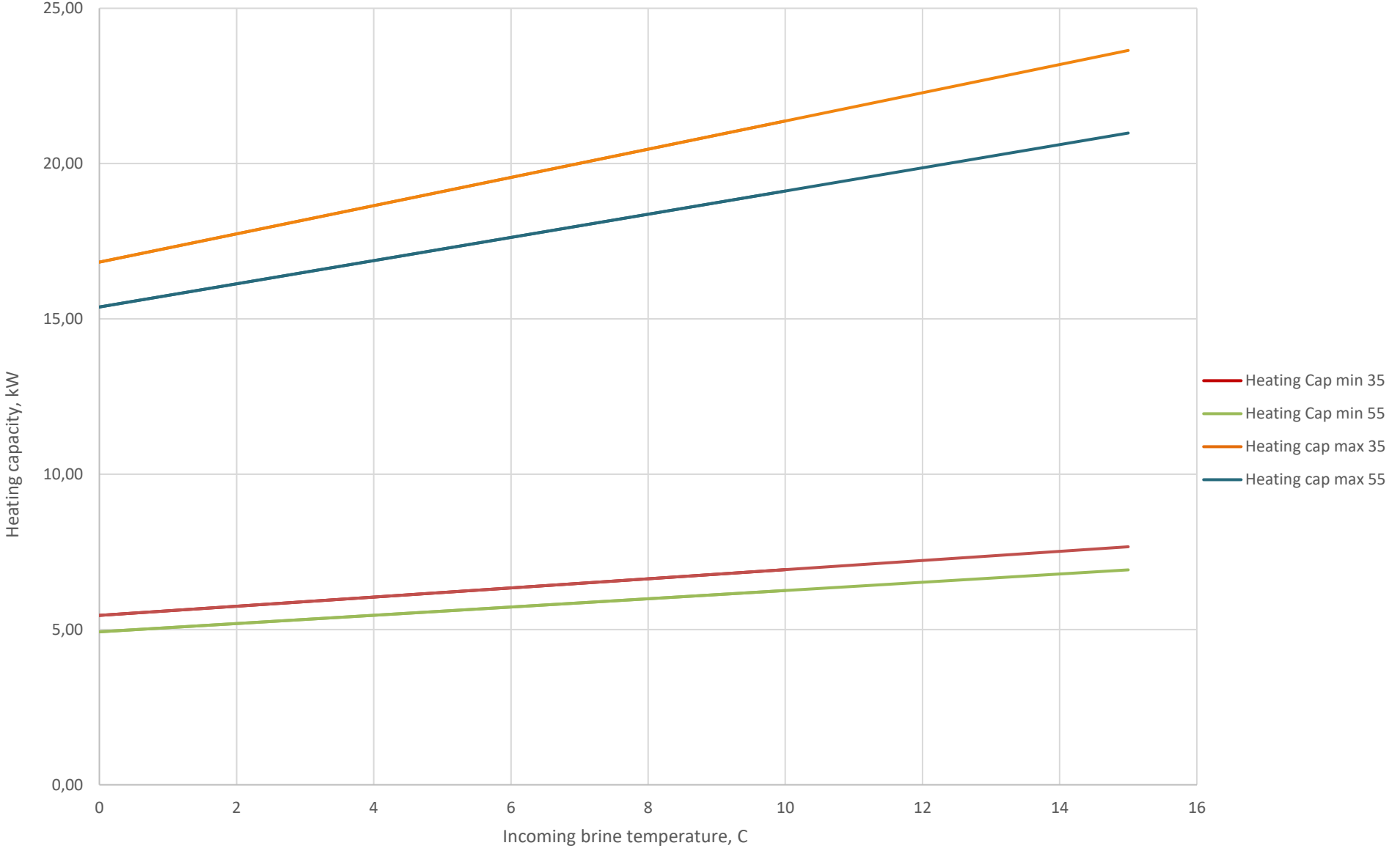
Heating capacity S1X55-16
