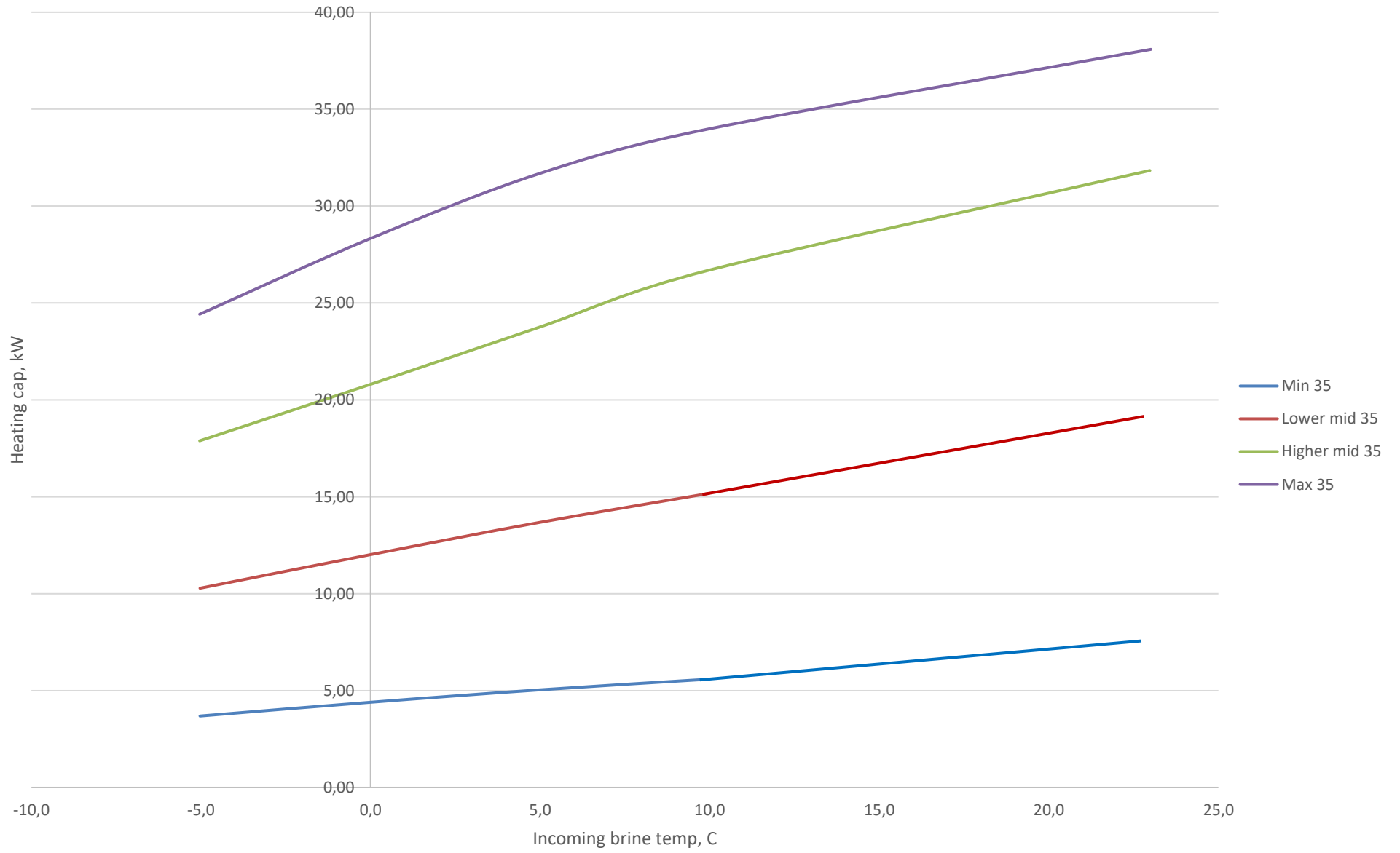
Heating cap F1355-28 @ 35 C supply temp
