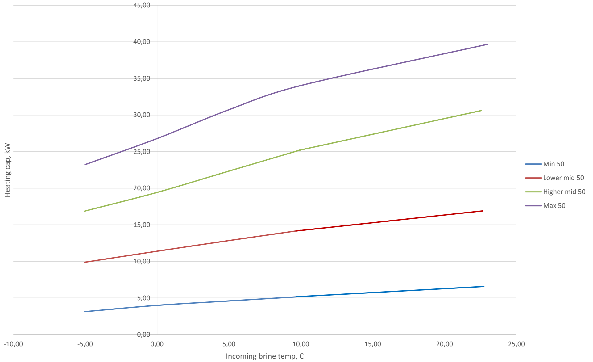
Heating cap F1355-28 @ 50 C supply temp
