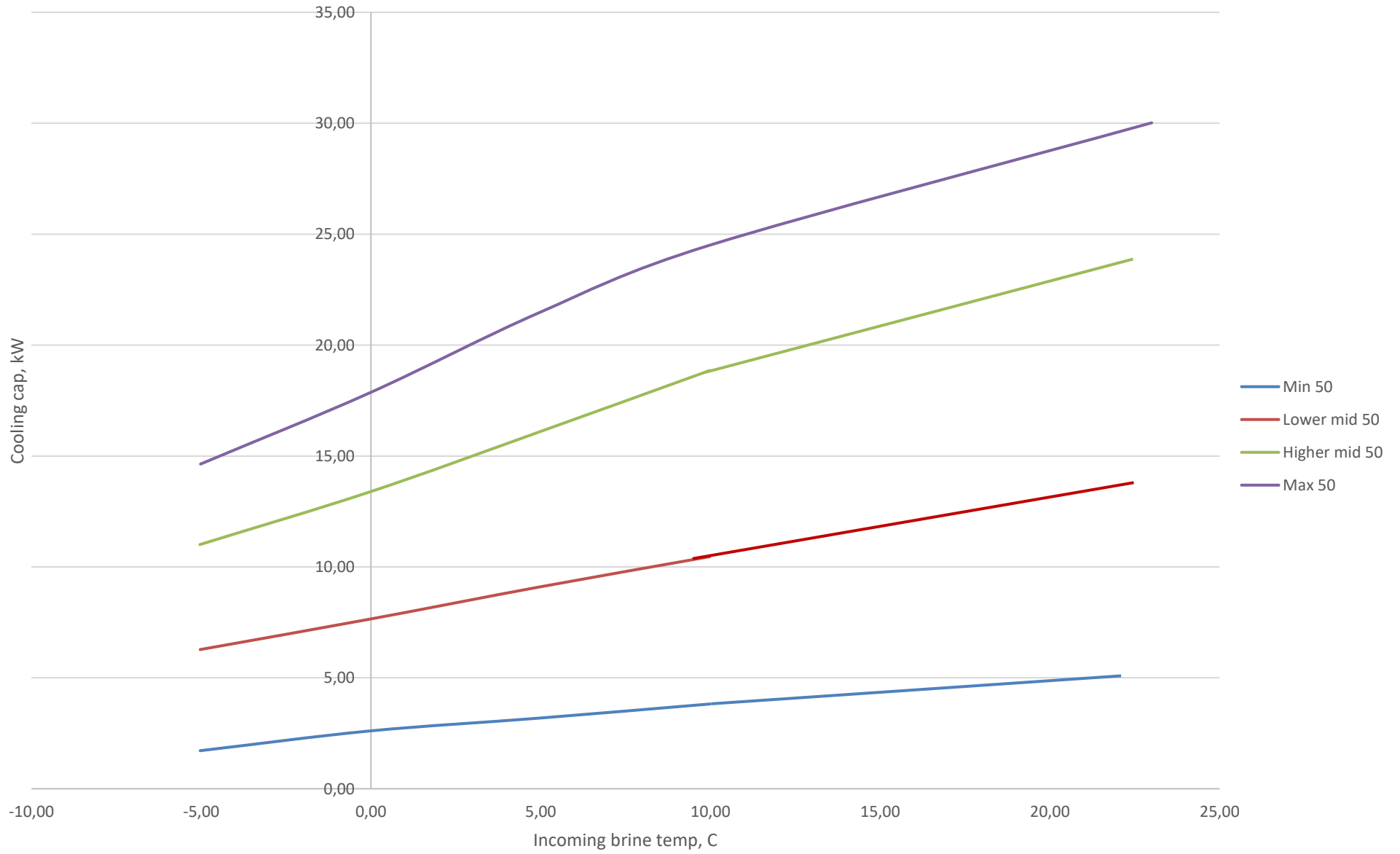
Cooling cap F1355-28 @ 50 C supply temp
