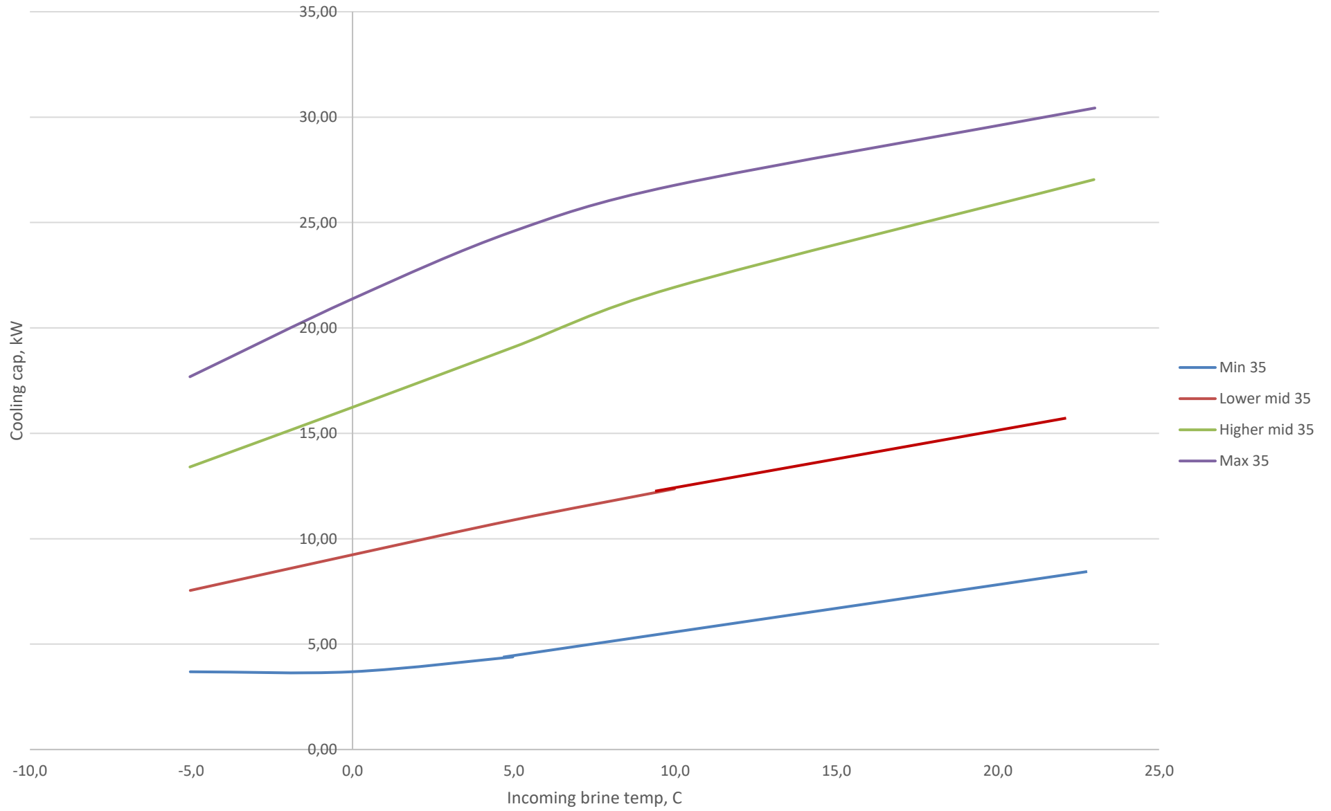
Cooling cap F1355-28 @ 35 C supply temp
