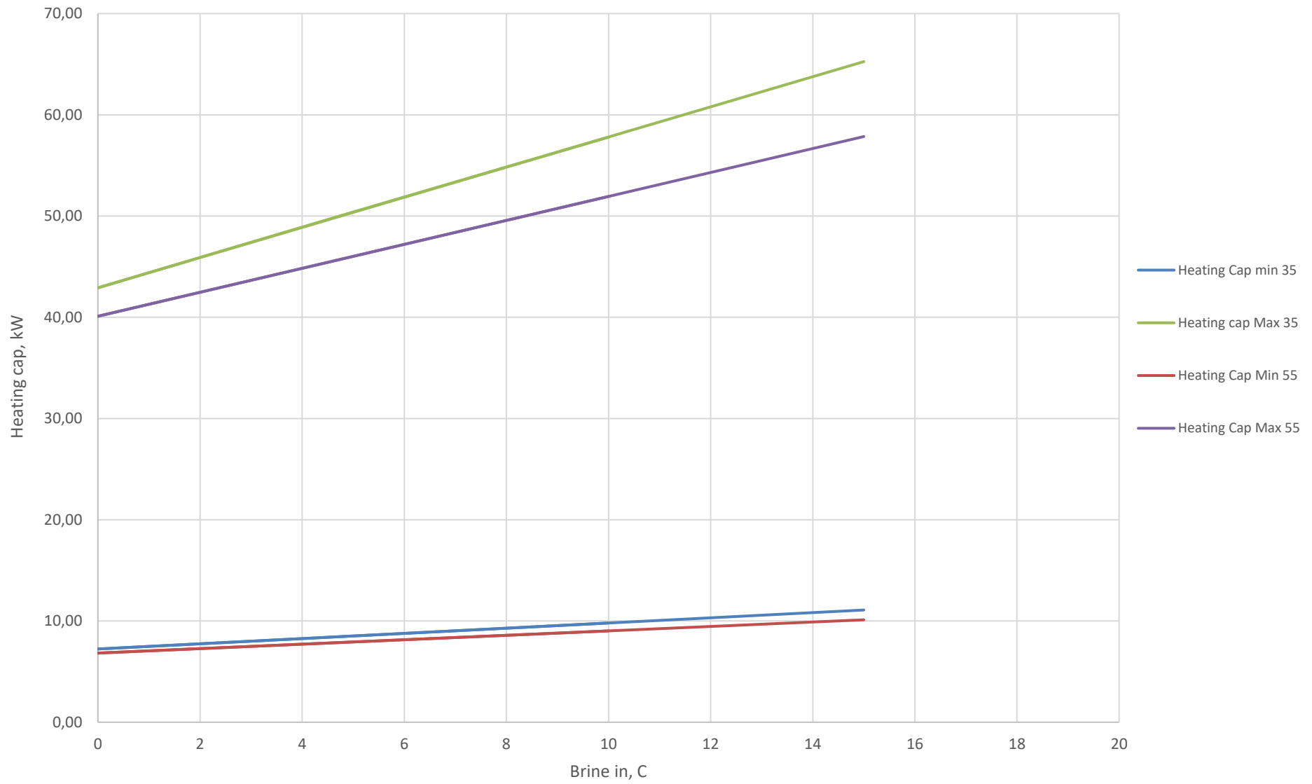
Heating cap F1355-43
