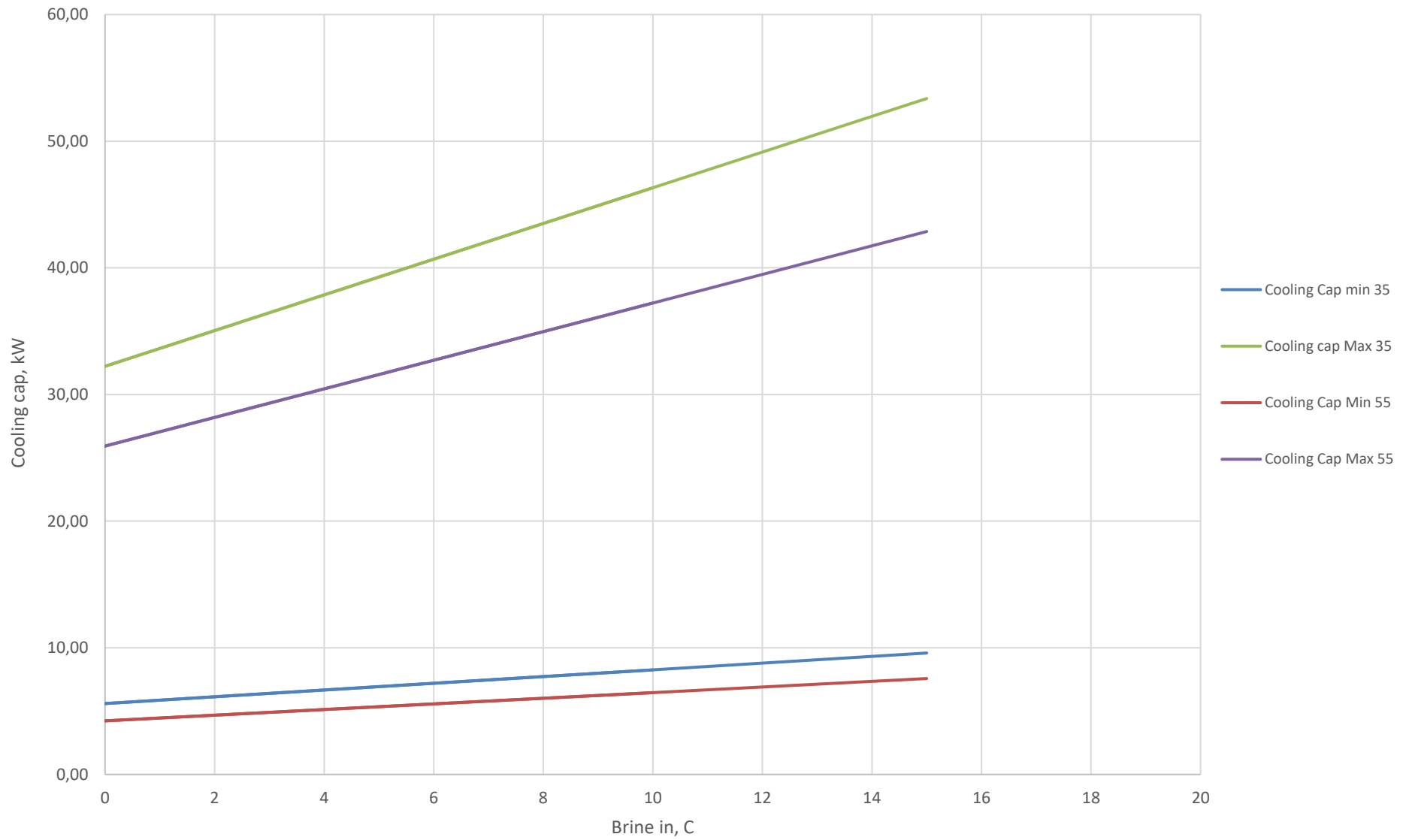
Cooling cap F1355-43
