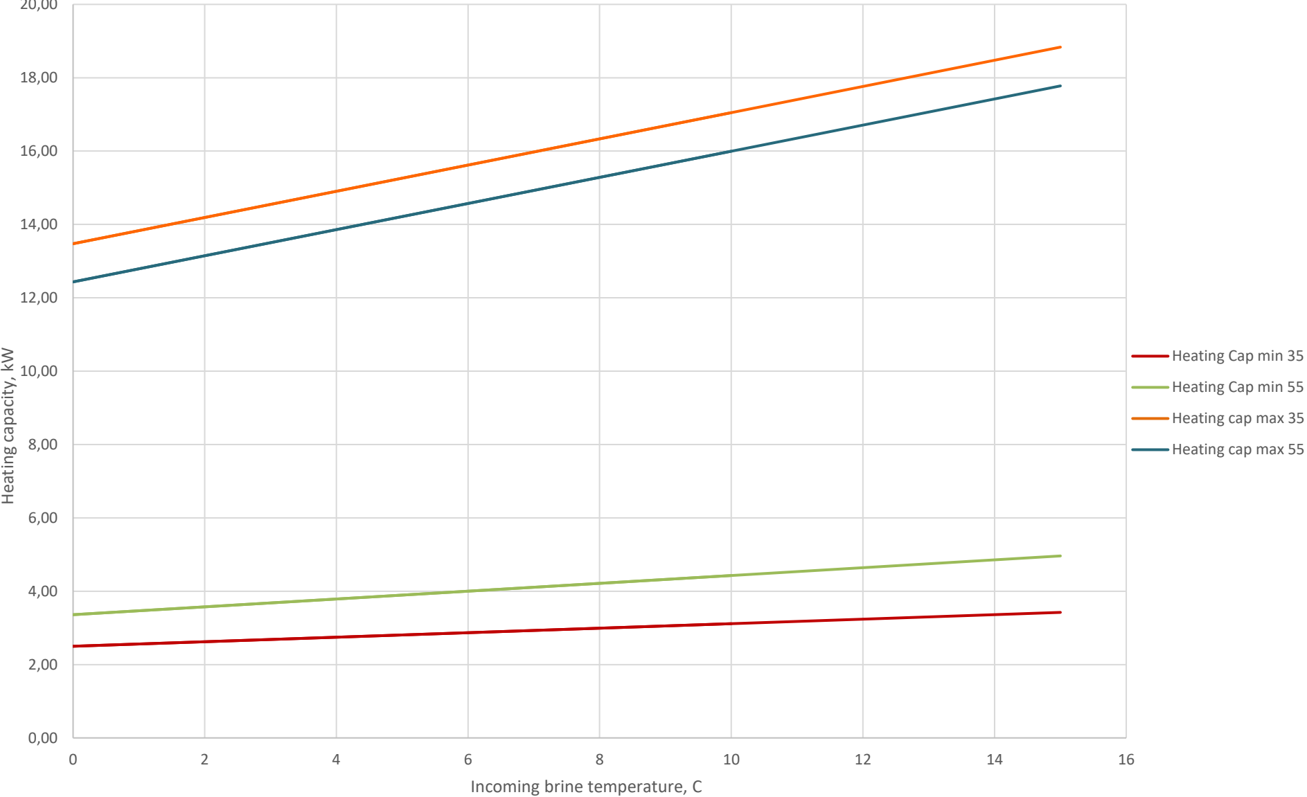
Heating capacity S1X55-12
