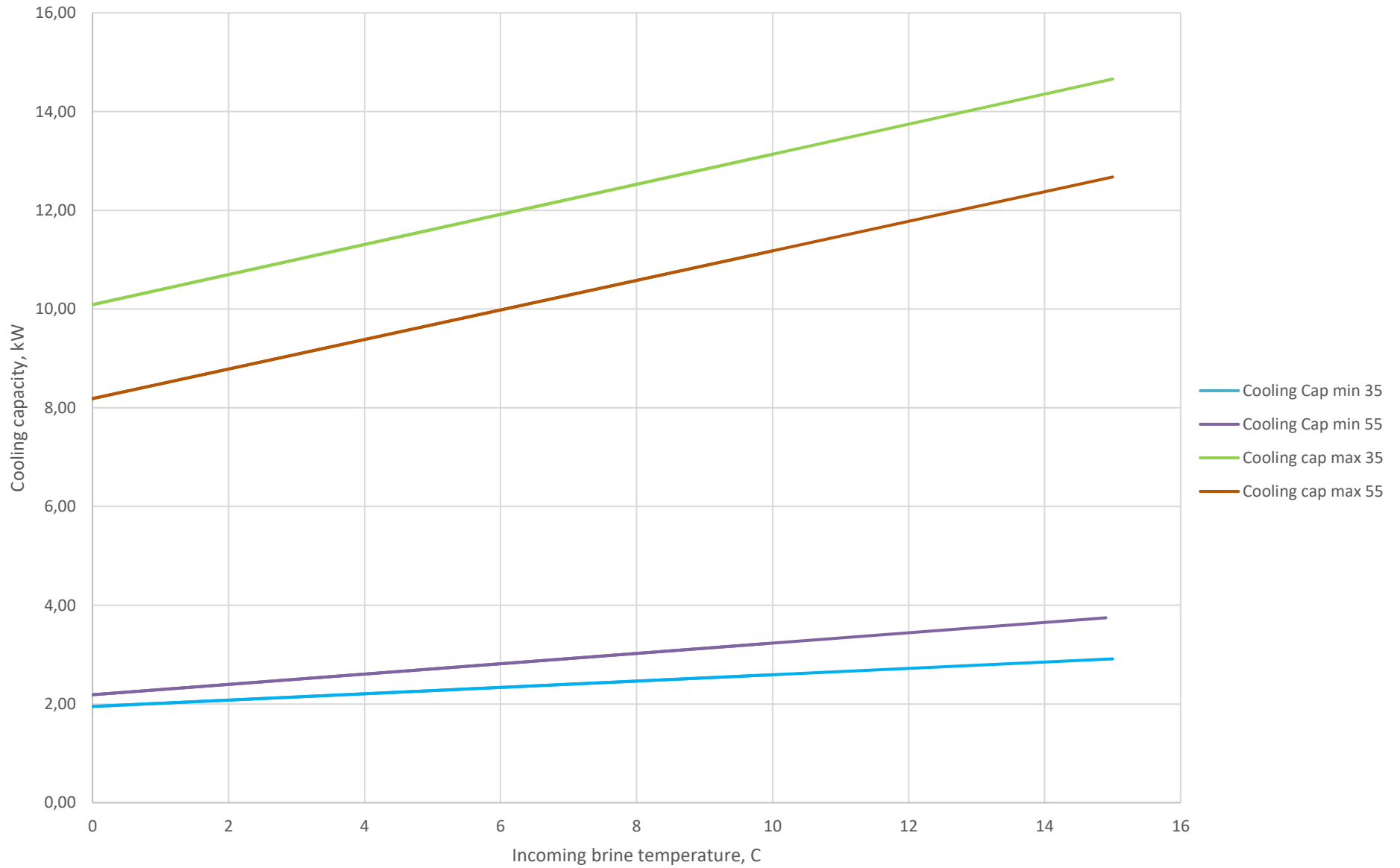
Cooling capacity S1X55-12
